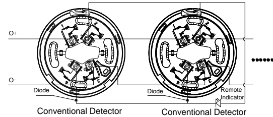
Figure 5 System Connection Diagram
